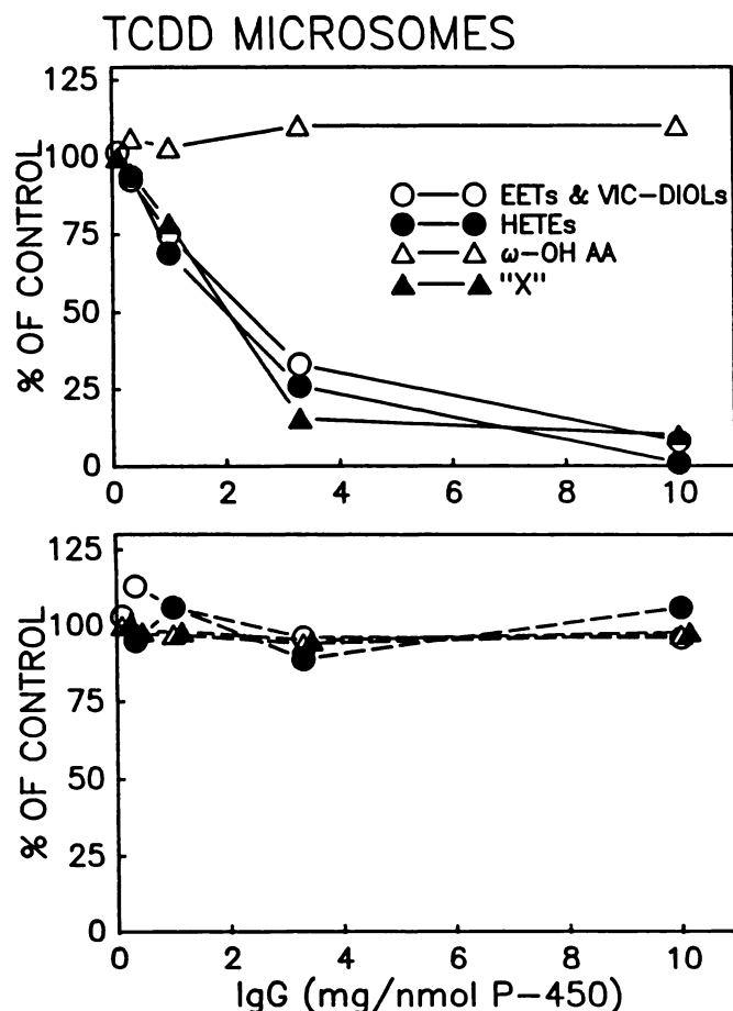
Fig. 5. Concentration-dependent effects of anti- \beta NF _{\alpha\alpha} IgG ( top ) and anti-PB P-450 IgG ( bottom ) on P-450-mediated arachidonic acid metabolism by liver microsomes from TCDD-treated chick embryos. Chick embryos were treated with TCDD as described in the legend to Fig. 4. Microsomes were preincubated for 15 min at room temperature without IgG or with preimmune or immune IgG in the concentrations shown on the abscissa . Then arachidonic acid metabolism was measured as described in Experimental Procedures. Preincubation and preimmune IgG had no effect. Mean values for product formation (nmol of product/mg of protein/min, mean \pm standard error, nine experiments) in the absence of immune IgG were 0.87 \pm 0.13 for EETs and vicinal diols (combined to reflect total epoxigenase activity), 0.15 \pm 0.03 for HETEs, 0.09 \pm 0.02 for X, and 0.40 \pm 0.02 for \omega -OH-arachidonic acid. ED_{50} values for immunoinhibition of arachidonic acid metabolites in TCDD-treated microsomes by anti- \beta NF _{\alpha\alpha} IgG (nmol of IgG/nmol of P-450) were 1.8 for EETs and vicinal diols, 1.1 for HETEs, and 1.6 for X.
