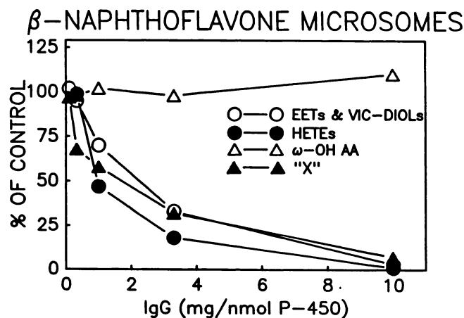
Fig. 6. Concentration-dependent immunoinhibition by anti- \beta NF _{\alpha\alpha} IgG of P-450-mediated arachidonic acid metabolism by microsomes from \beta NF-treated chick embryos. The procedures were the same as described in the legend to Fig. 5, except that the embryos were treated for 48 hr with 6.7 mg of \beta NF in 0.1 ml of dimethylsulfoxide. Mean values for product formation (nmol of product/mg of protein/min, mean \pm standard error, six experiments) in the absence of immune IgG were 0.73 \pm 0.03 for EETs and vicinal diols, 0.08 \pm 0.01 for HETEs, 0.08 \pm 0.01 for X, and 0.4 \pm 0.02 for \omega -OH-arachidonic acid. The ED_{50} values for immunoinhibition of arachidonic acid metabolites in \beta NF-treated microsomes by anti- \beta NF _{\alpha\alpha} IgG were 1.7 for EETs and vicinal diols, 1.4 for HETEs, and 1.2 for X.
