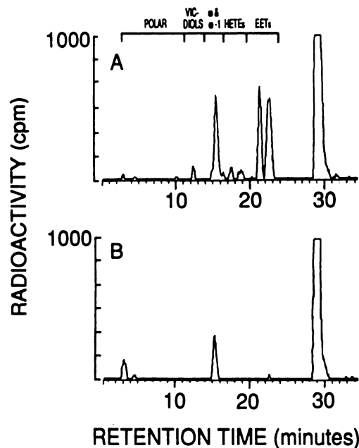
Fig. 7. Reverse phase HPLC chromatograms showing immunoinhibition by anti-PB IgG of PB-induced arachidonic acid metabolism. Liver microsomes (1.37 nmol of P-450/mg of microsomal protein) from chick embryos 48 hr after treatment with 20 mg of sodium PB were preincubated for 15 min at room temperature without IgG (A) or with anti-PB IgG (B) at 10 mg of IgG/nmol of P-450. Arachidonic acid metabolism, product extraction, and resolution by reverse phase HPLC were performed as described in Experimental Procedures. Arachidonic acid products formed in the absence of immune serum (nmol of product/mg of protein/min, means of duplicate determinations) for the sample shown were 0.74 for EETs, 0.09 for HETEs, 0.27 for \omega -OH-arachidonic acid, and 0.05 for vicinal diols. The samples shown in A and B contained 197,609 and 131,023 cpm of ^{14} C, respectively.
